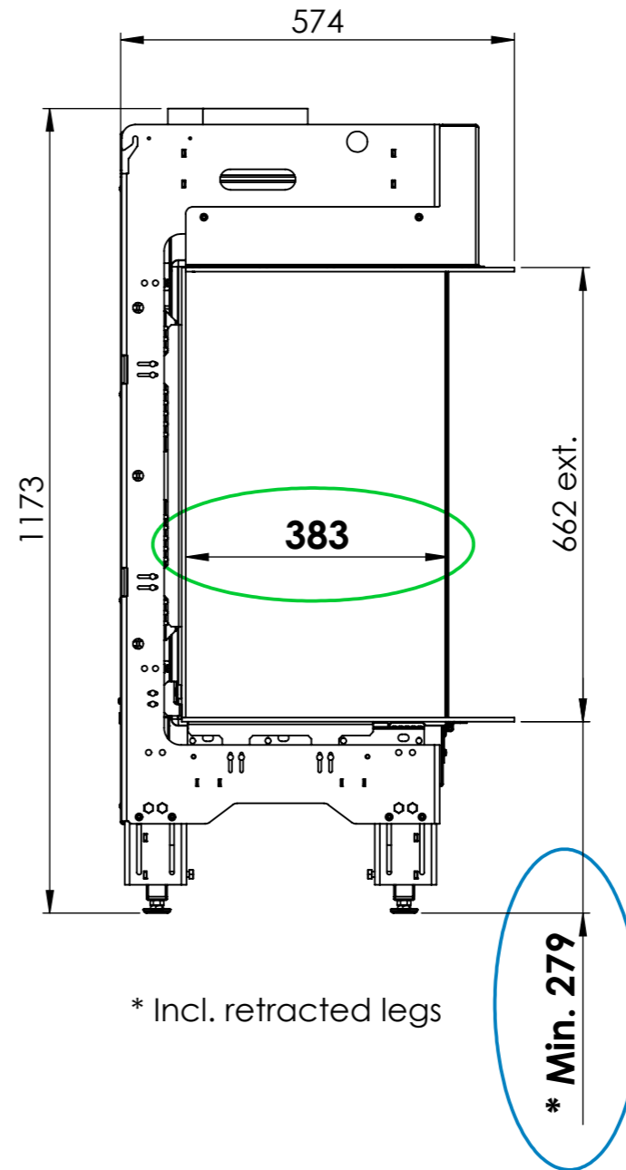
MatriX Hybrid 800x650 I, II, III (Logburner 3.0)
